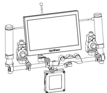
Configuration Example #3: Flying / Without Shoulder Mount
